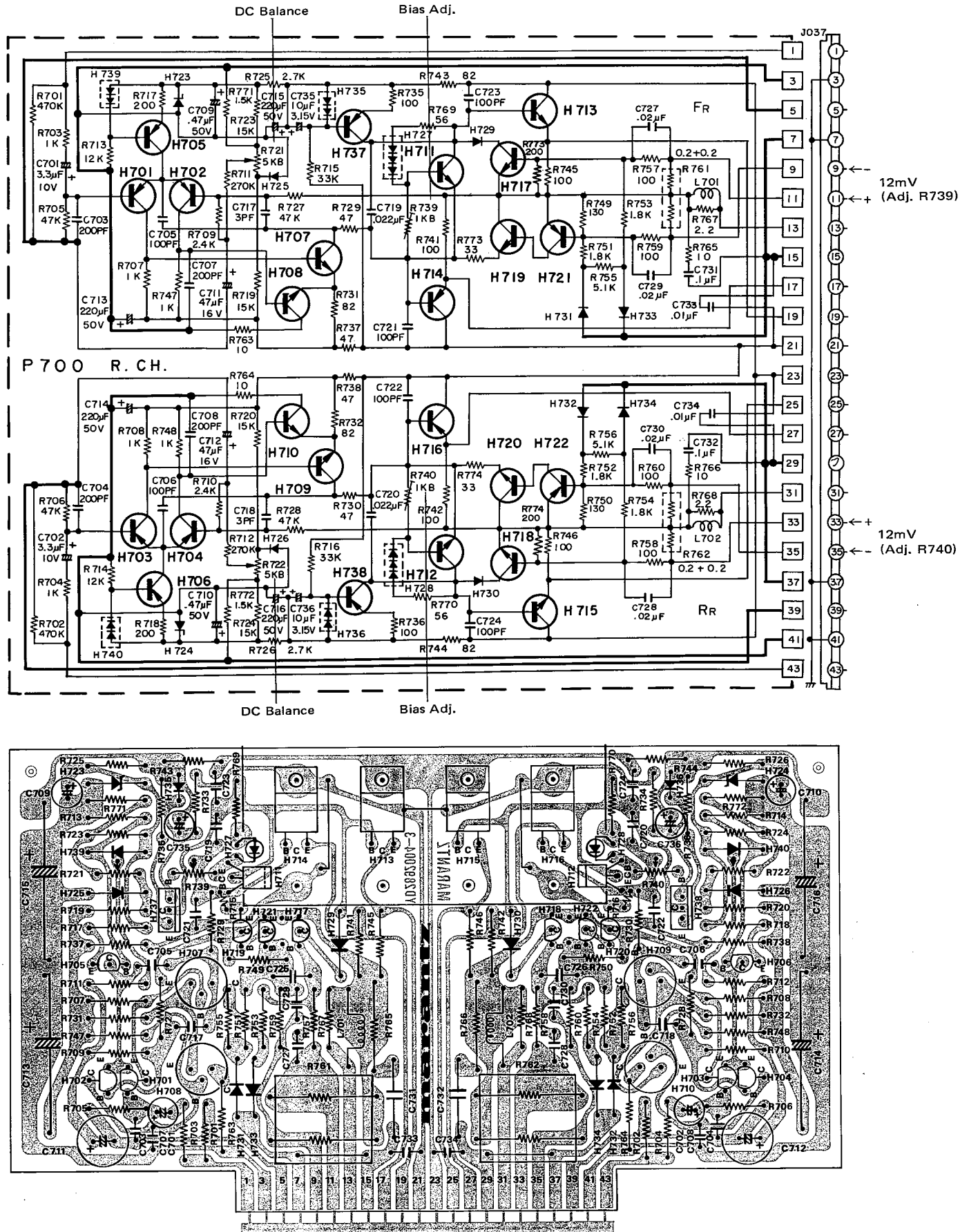
Figure 15. Power Amplifier Assembly P700 Component Locations and Schematic Diagram
